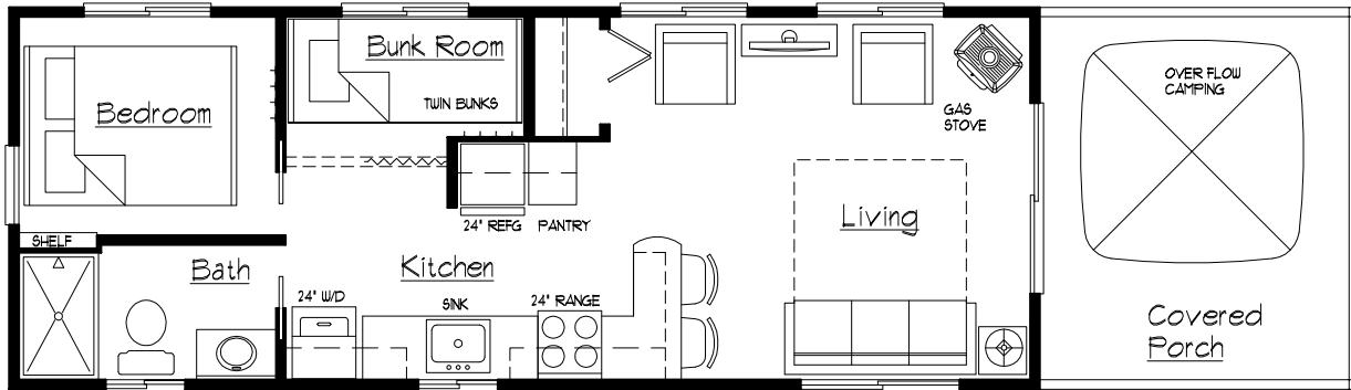
Concept Plan 112 - 12'-0"
