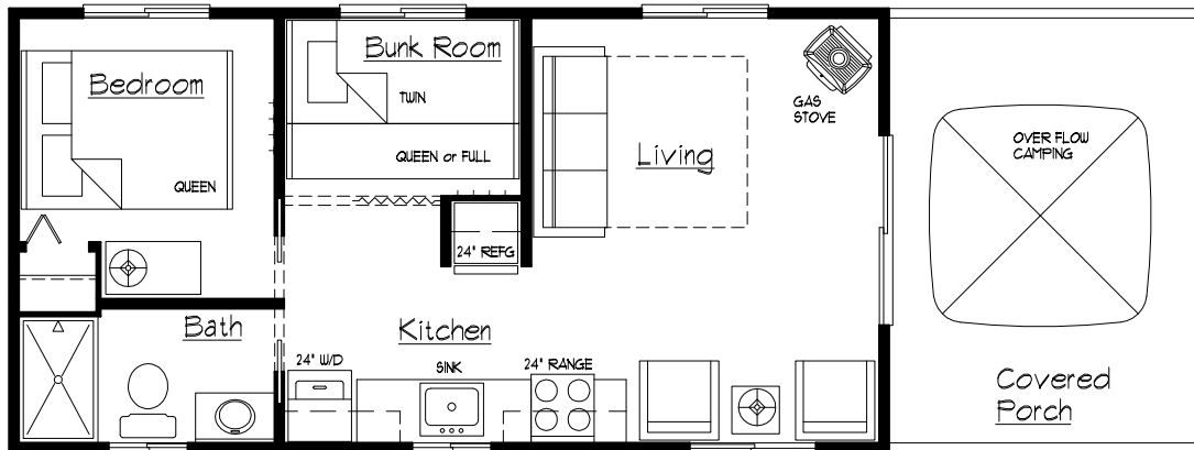
Concept Plan 112 - 14'-0"
